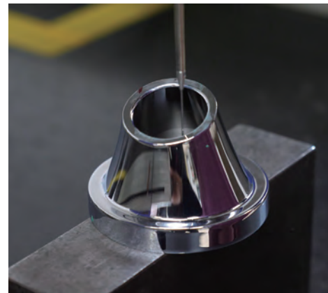
3D CMM Dimention Measurement
